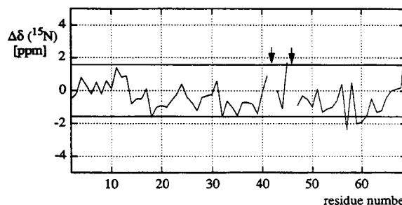
Figure 3. Plot versus the amino acid sequence of the differences between the ^{15}\text{N} chemical shifts measured for the unfolded DNA-binding domain of the 434 repressor in 7 M urea at pH 4.8 and the "random coil" reference shifts predicted using eq 1 and Table 2. The values for Glu and Asp were interpolated (Table 2). The arrows identify the positions of Pro 42 and Pro 46 for which no ^{15}\text{N} chemical shifts are available. The two solid lines indicate the chemical shift range of \pm 1.6 ppm (see text). The experimental shifts from the 434 repressor were recalibrated to the presently used external liquid \text{NH}_3 reference by the addition of 1.3 ppm to the values reported in ref 7.
